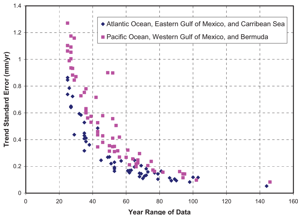
Figure B-2. Standard Error of Linear Trend of Sea-level rise vs. Period of Record, U.S. Tide Stations.
